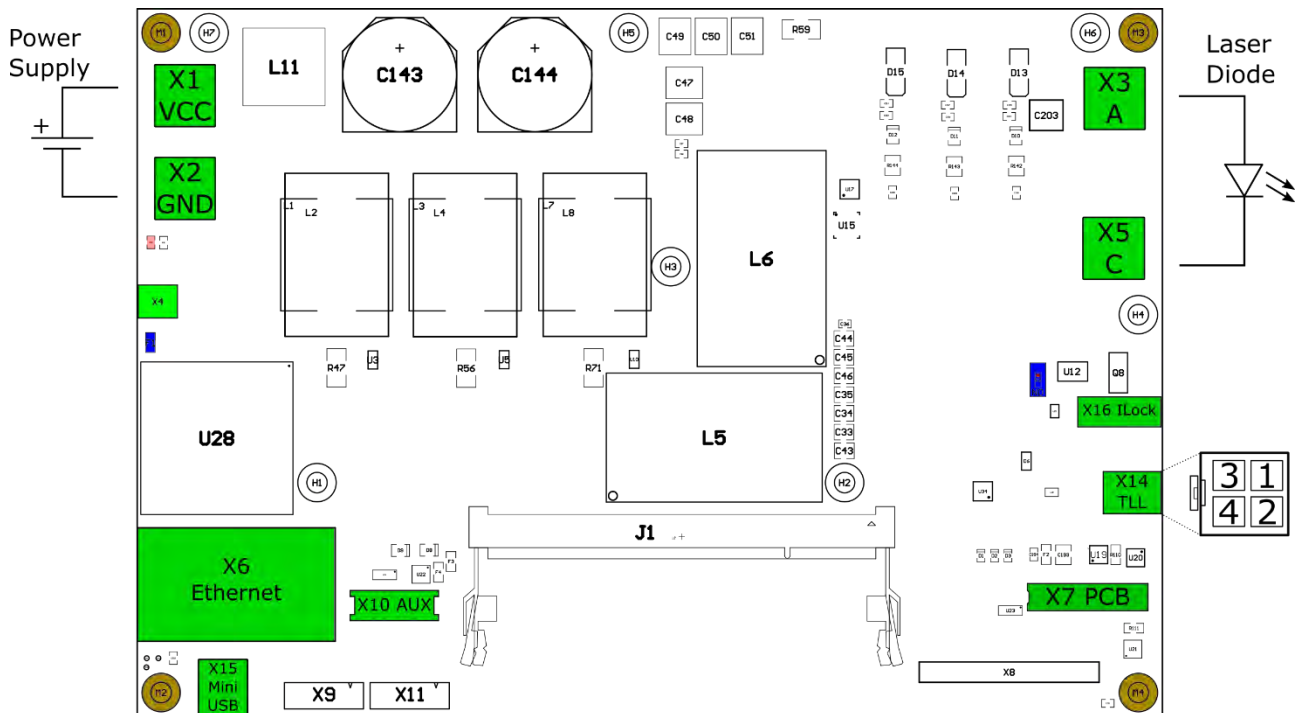
Top view
