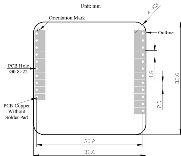
Figure 21. Top View of the Top Side PCB Foot-print
