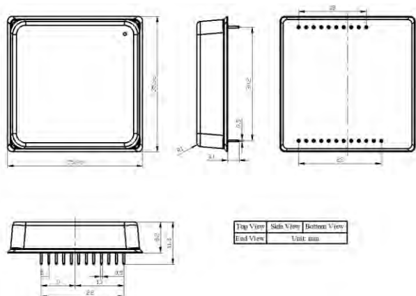
Figure 19. Dimensions of the DIP Package Driver
