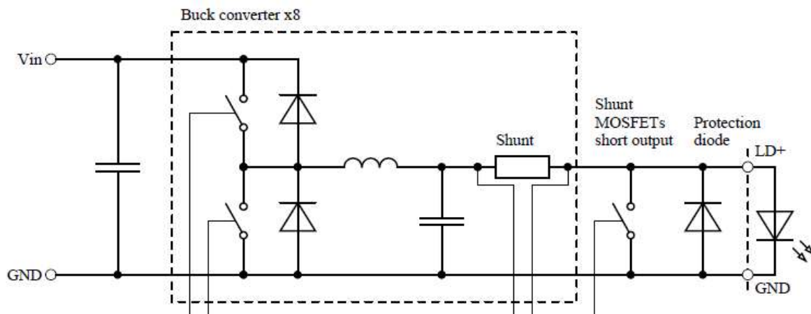
Figure 10 – Analog interface functional scheme
