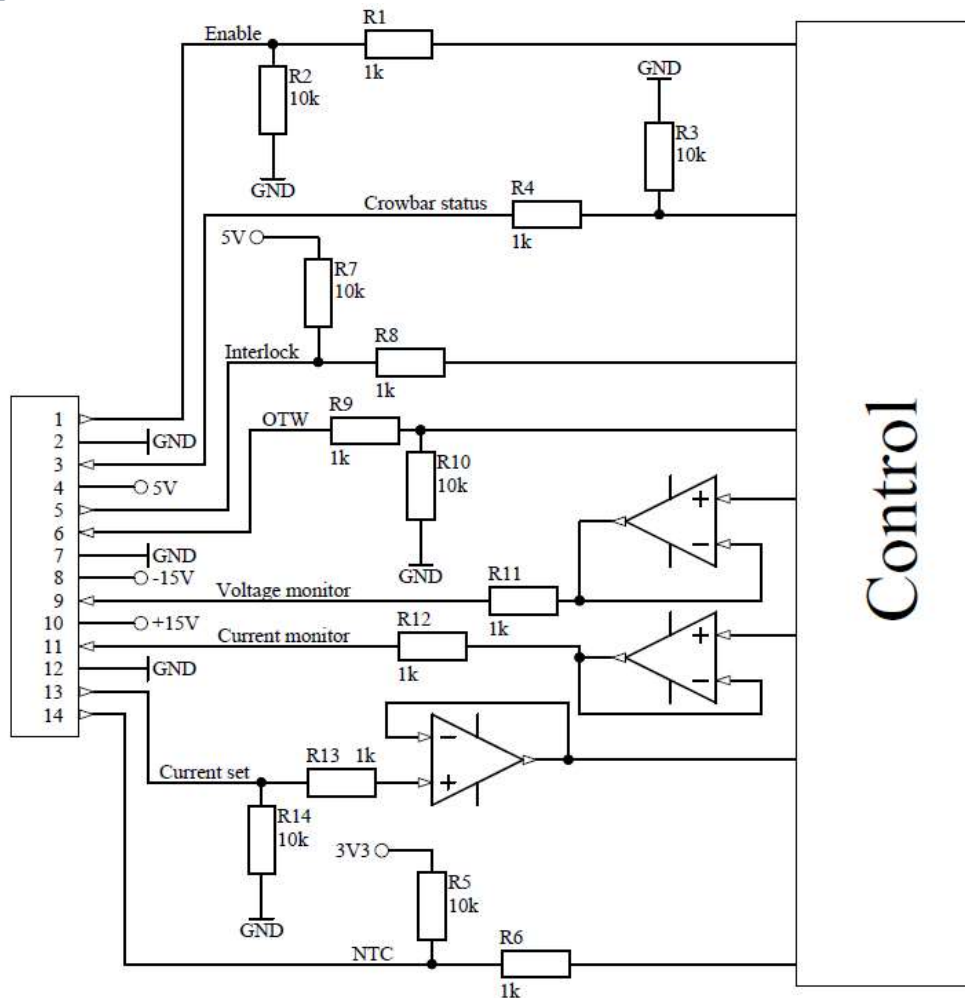
Figure 10 – Analog interface functional scheme
