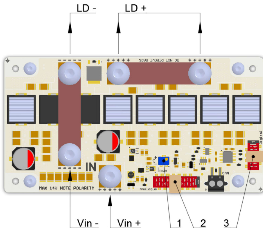
Figure 12 – Terminals and controls
