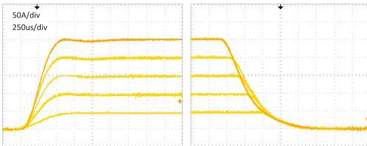
Figure 7 – Typical start up and stop sequence at V_{out} = 1.8-2.3V
