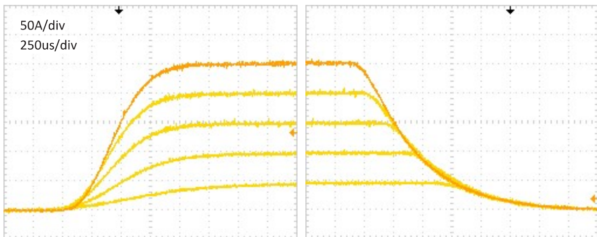
Figure 9 – Typical start up and stop sequence at V_{out} = 6.9-9.0V
