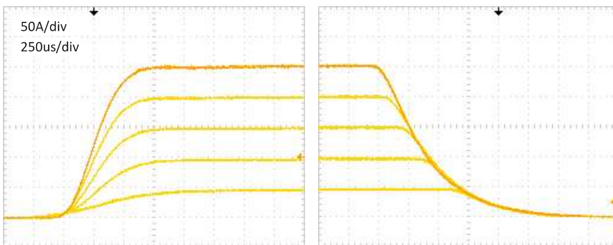
Figure 8 – Typical start up and stop sequence at V_{out} = 4.3-5.4V
