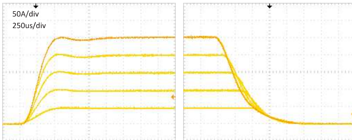
Figure 6 – Typical start up and stop sequence at V_{out} = 0.9-1.3V
