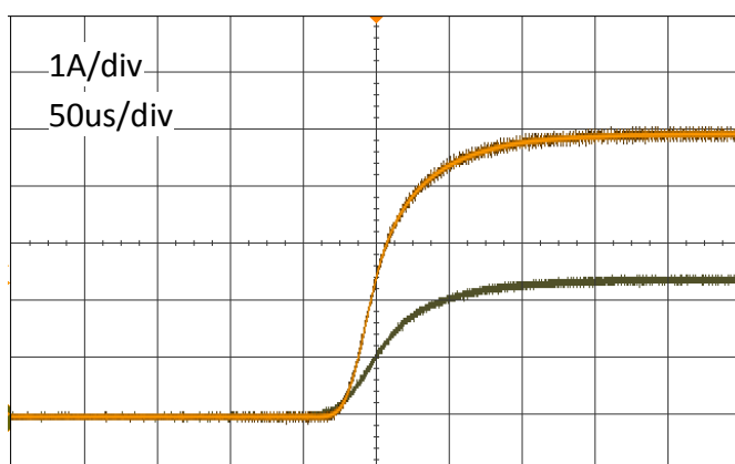
Figure 3 – Typical start up sequence
