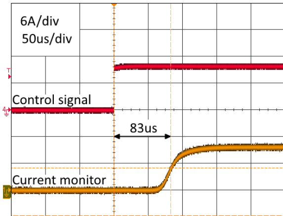
Figure 20 – Typical delay between Current Set control signal and current pulse, 10A @ 500Hz
