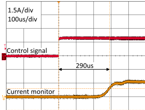
Figure 18 – Typical delay between Current Set control signal and current pulse, 2A @ 500Hz
