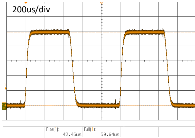
Figure 10 – 15A @ 10V @ 1kHz
