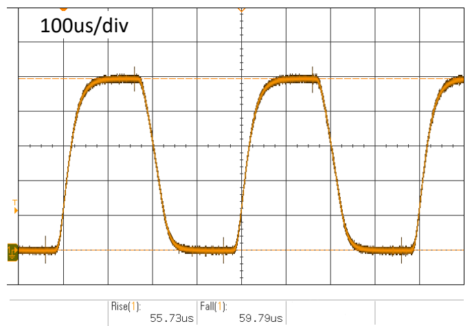
Figure 7 – 15A @ 40V @ 2.5kHz
