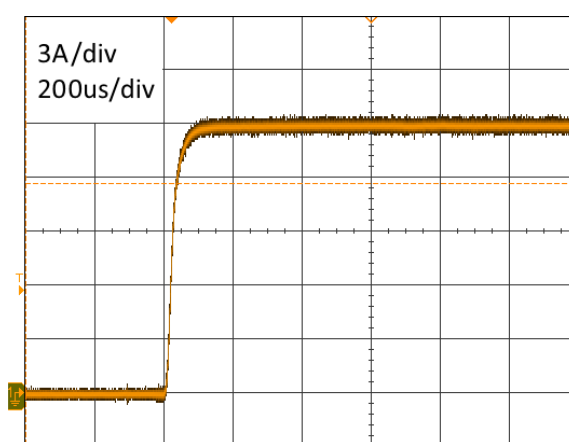
Figure 15 – Typical pulse edge with Current Set control signal
