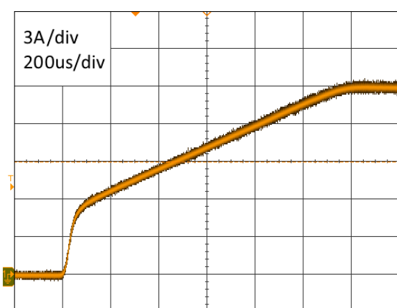
Figure 14 – Typical pulse edge with Enable control signal
