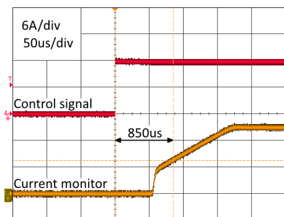
Figure 16 – Typical delay between Enable control signal and current pulse, 15A @ 500 Hz
