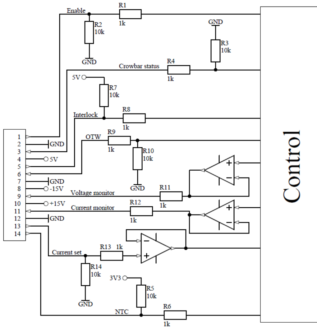
Figure 24 – Analog interface functional scheme
