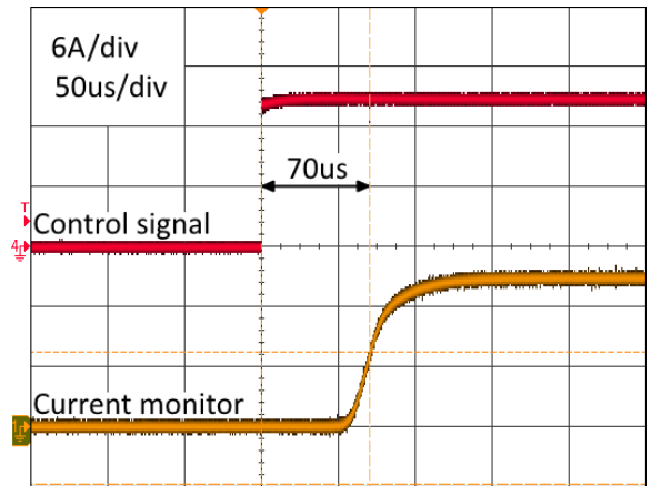
Figure 21 – Typical delay between Current Set control signal and current pulse, 15A @ 500Hz
