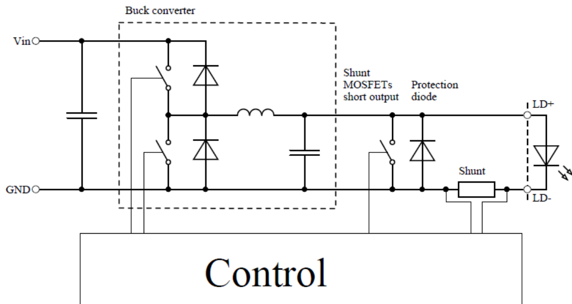
Figure 25 – Power unit functional scheme
