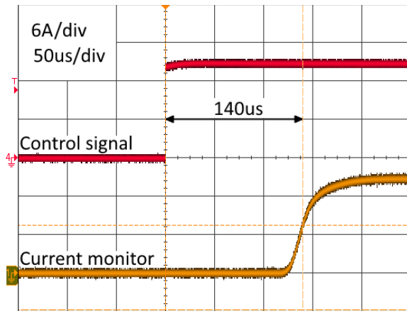
Figure 22 – Typical delay between Current Set control signal and current pulse, 15A @ 10Hz
