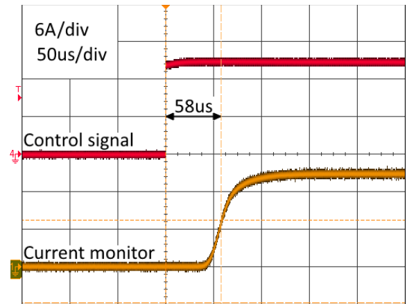
Figure 23 – Typical delay between Current Set control signal and current pulse, 15A @ 1000Hz
