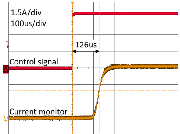
Figure 19 – Typical delay between Current Set control signal and current pulse, 5A @ 500Hz
