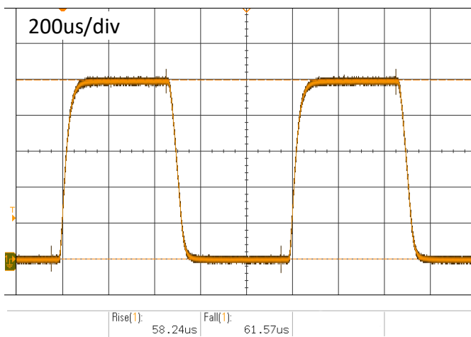
Figure 6 – 15A @ 40V @ 1kHz
