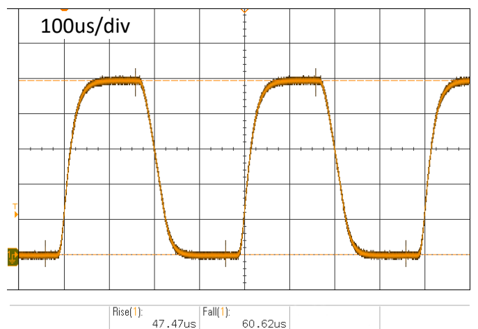
Figure 9 – 15A @ 20V @ 2.5kHz
