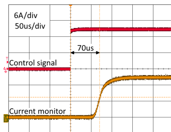
Figure 17 – Typical delay between Current Set control signal and current pulse, 15A @ 500 Hz
