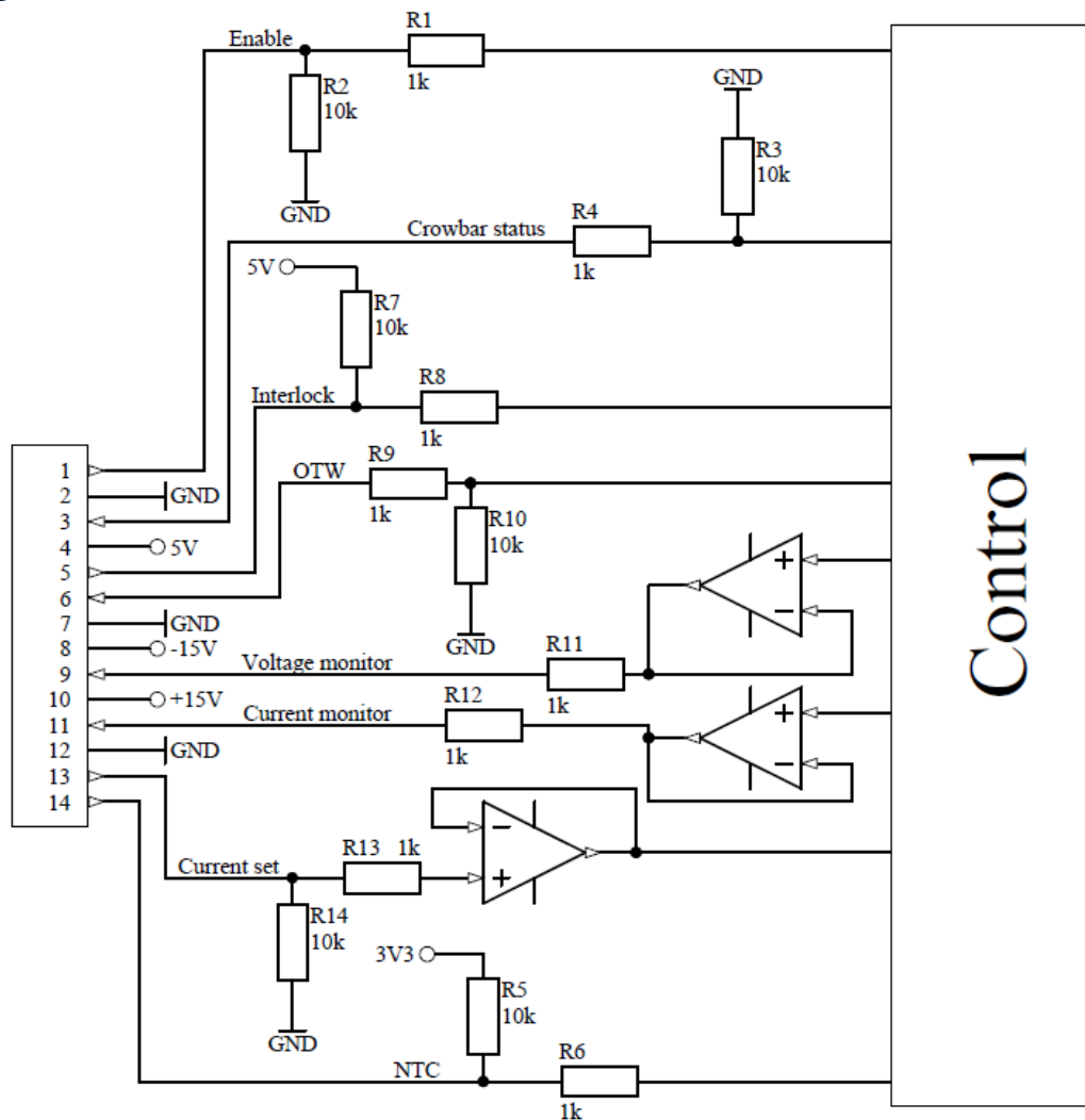
Figure 10 – Analog interface functional scheme
