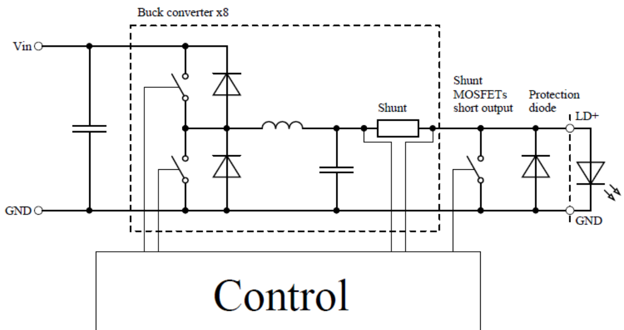
Figure 11 – Power unit functional scheme
