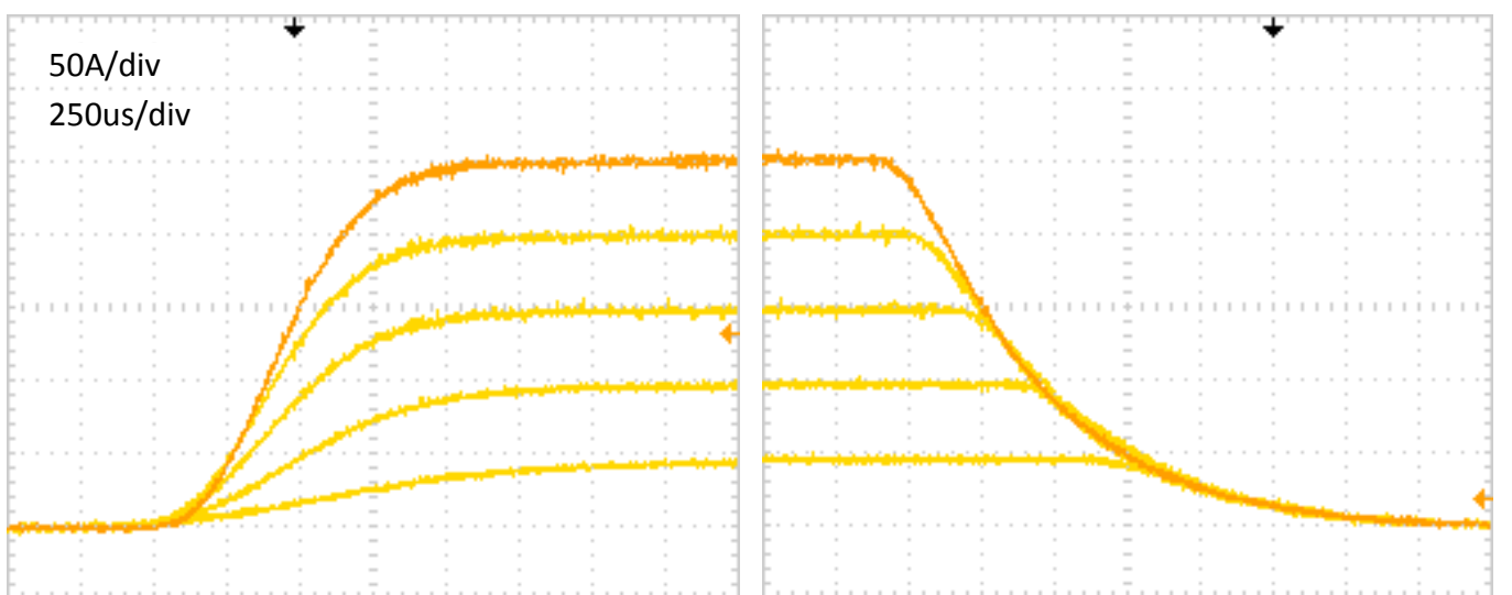
Figure 9 – Typical start up and stop sequence at V_{out} = 6.9-9.0V
