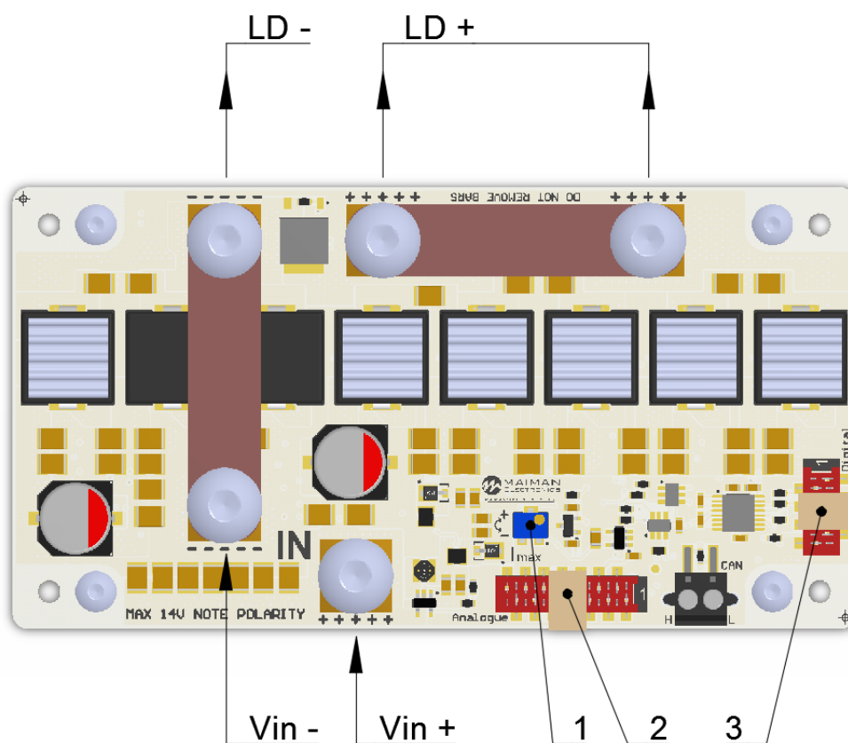
Figure 12 – Terminals and controls
