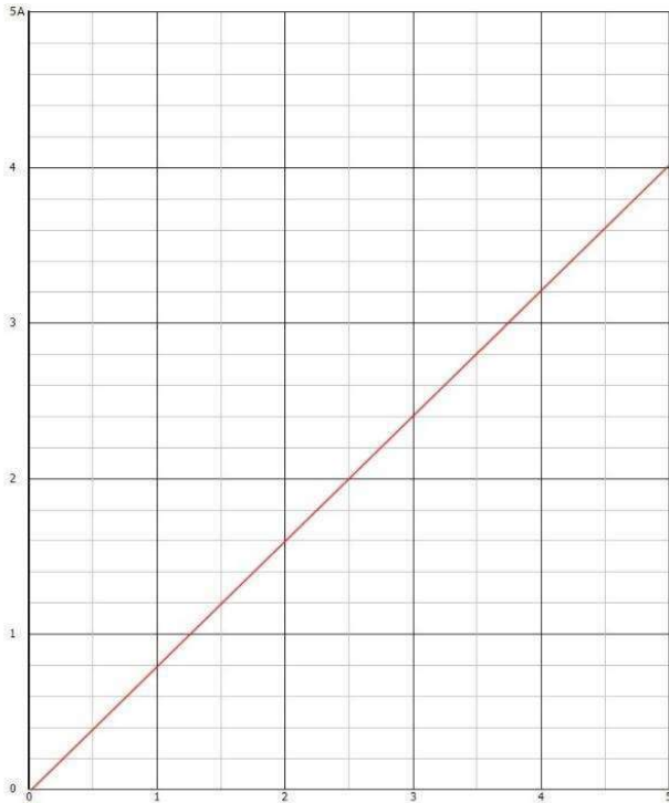
Figure 1. Characteristic with no offset current ("Offset jumper" removed). Maximum output current 4A.
