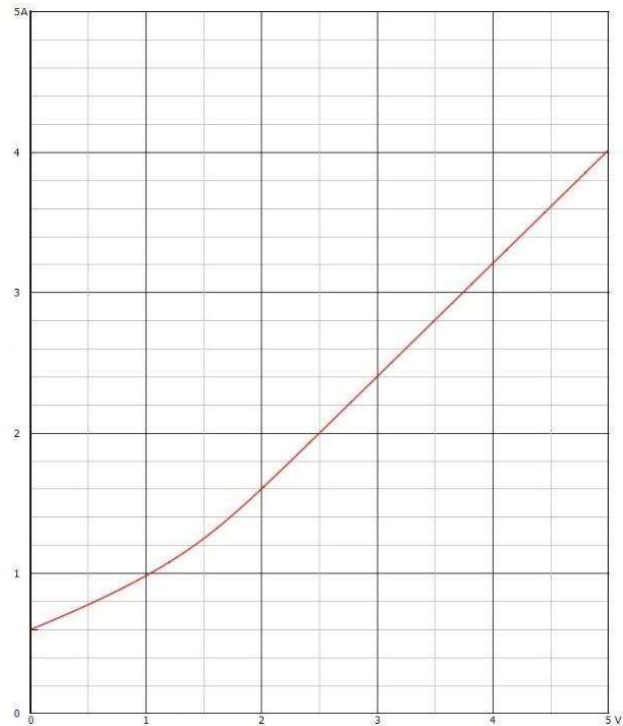
Figure 2. Characteristic with an offset current 0.6A ("Offset jumper" placed). Maximum output current 4A.
