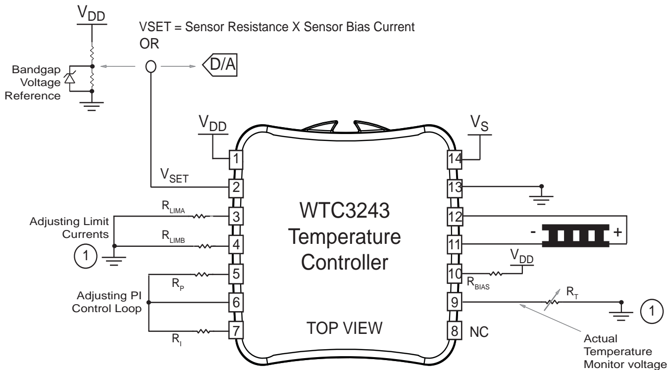
Figure 3. WTC3243 Quick Connect for TEC with Thermistor
