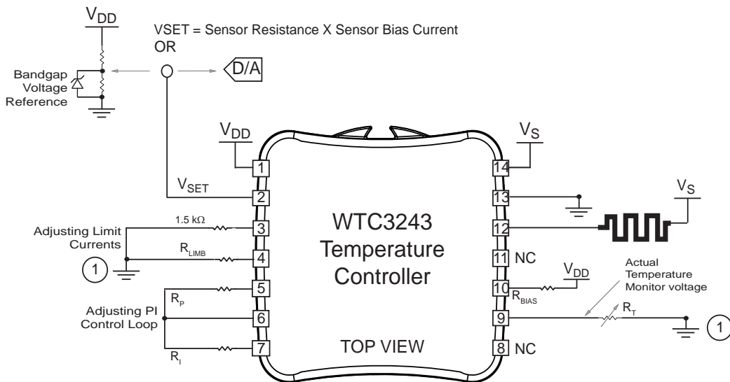
Figure 16. Thermistor / TEC Operation -- Top View
