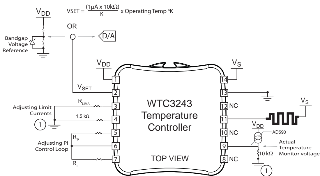
Figure 23. AD590 / Resistive Heater Operation -- Top View
