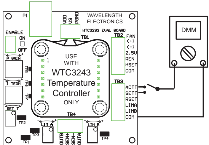
Figure 15. WTC3243 Evaluation Board & Voltmeter
