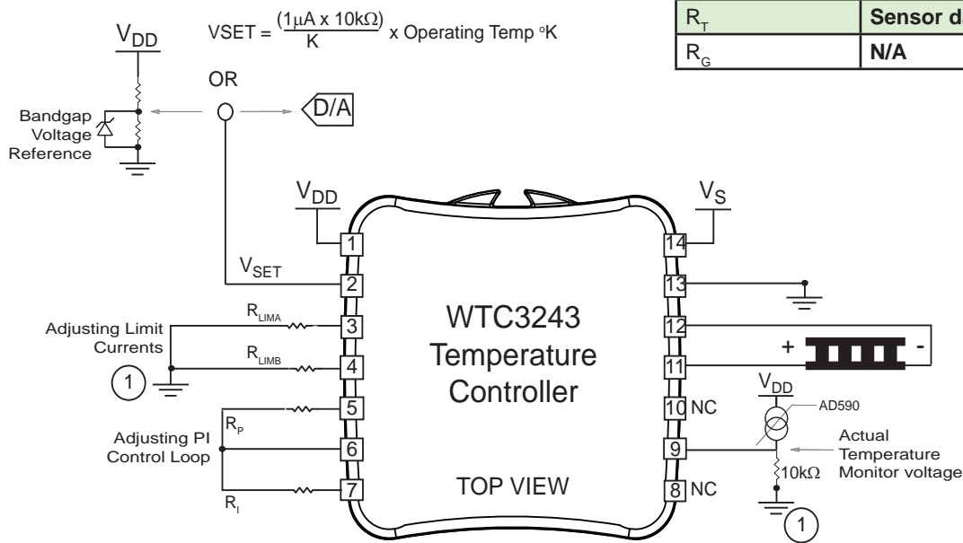
Figure 22. AD590 / Thermoelectric Operation -- Top View
