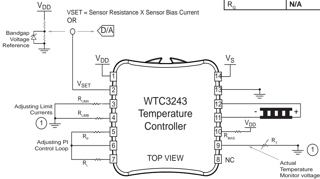
Figure 16. Thermistor / TEC Operation -- Top View
