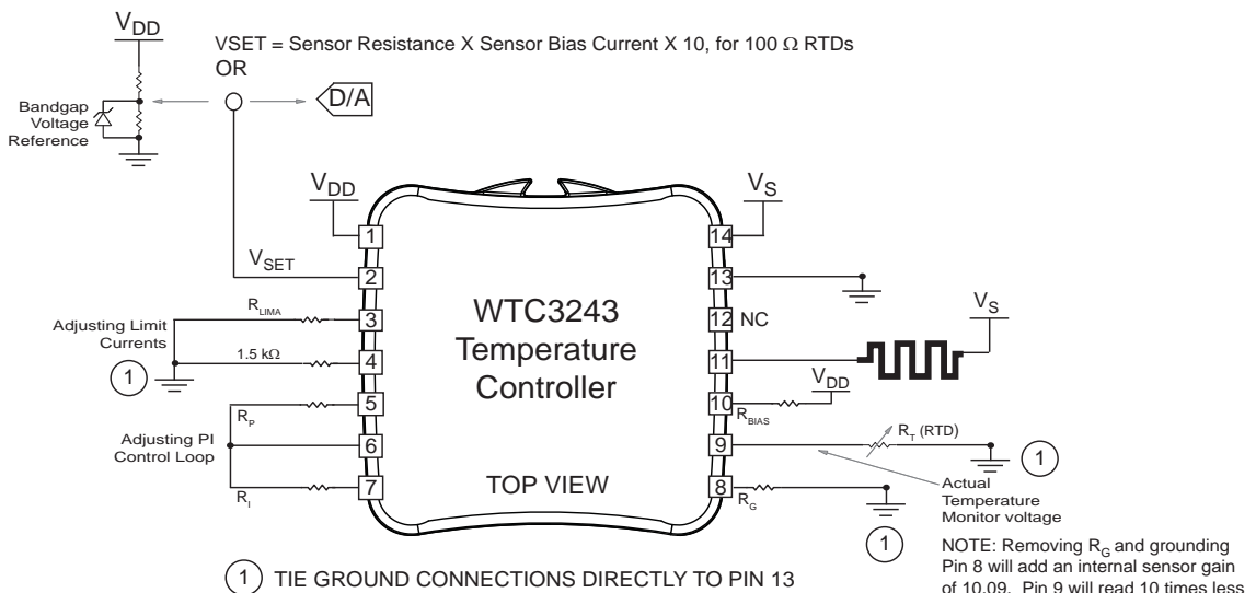
Figure 19. RTD / Resistive Heater Operation -- Top View
