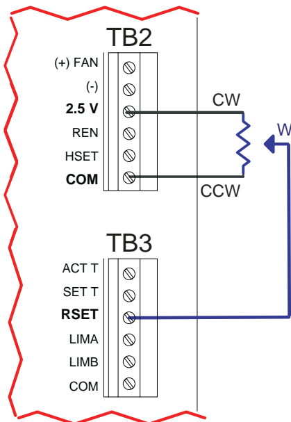
Figure 28. Example Wiring—External RSET Adjustment
