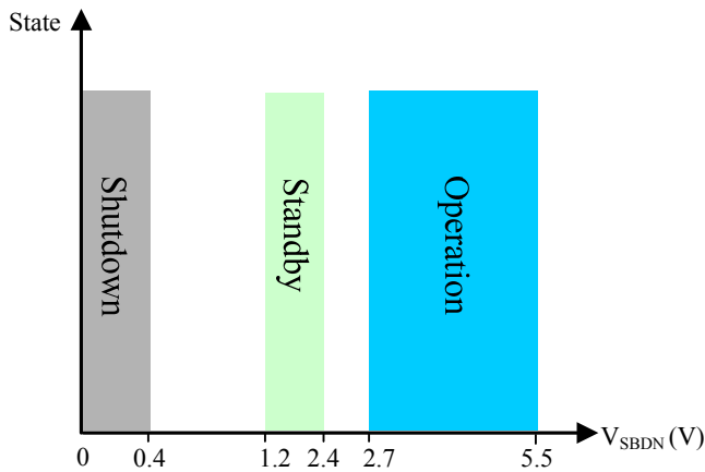
Figure 3. Input Control
