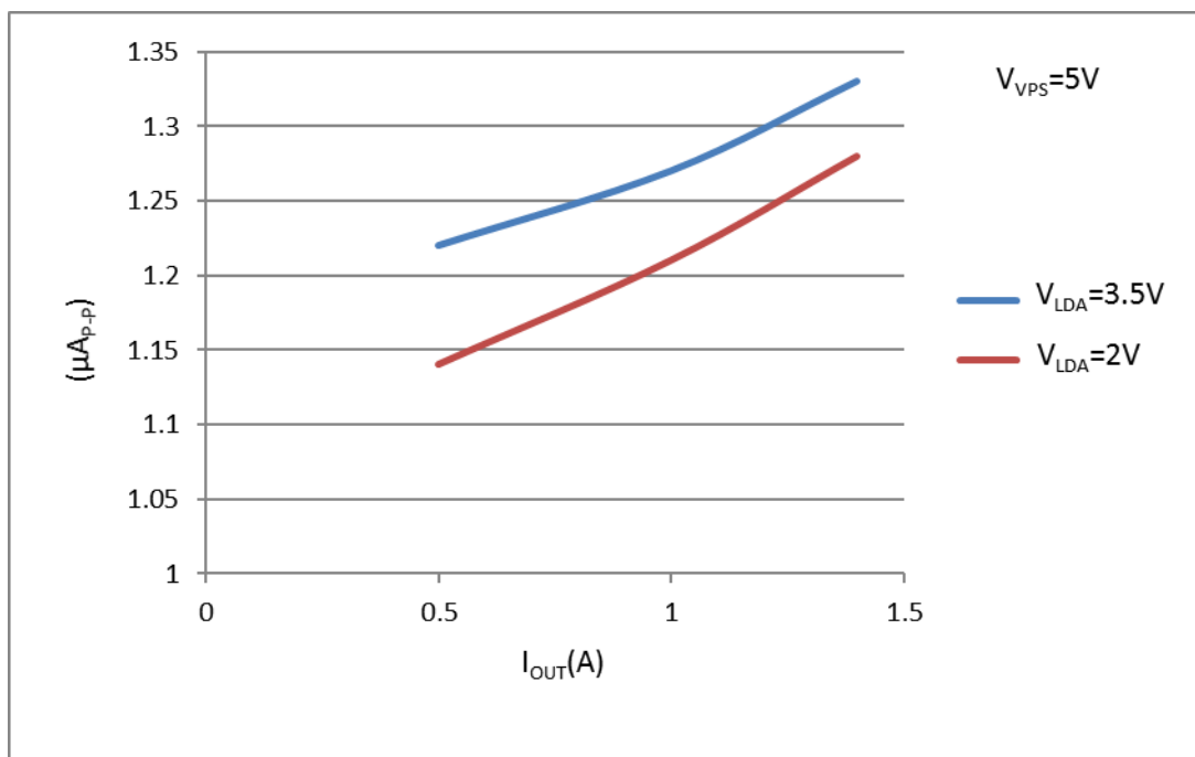
Figure 11.2. I_{OUT} vs. Output Current Noise@0.1Hz~10Hz
