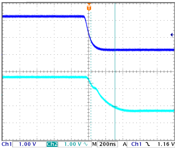
Figure 12.2. Large Signal Fall Time 280ns
