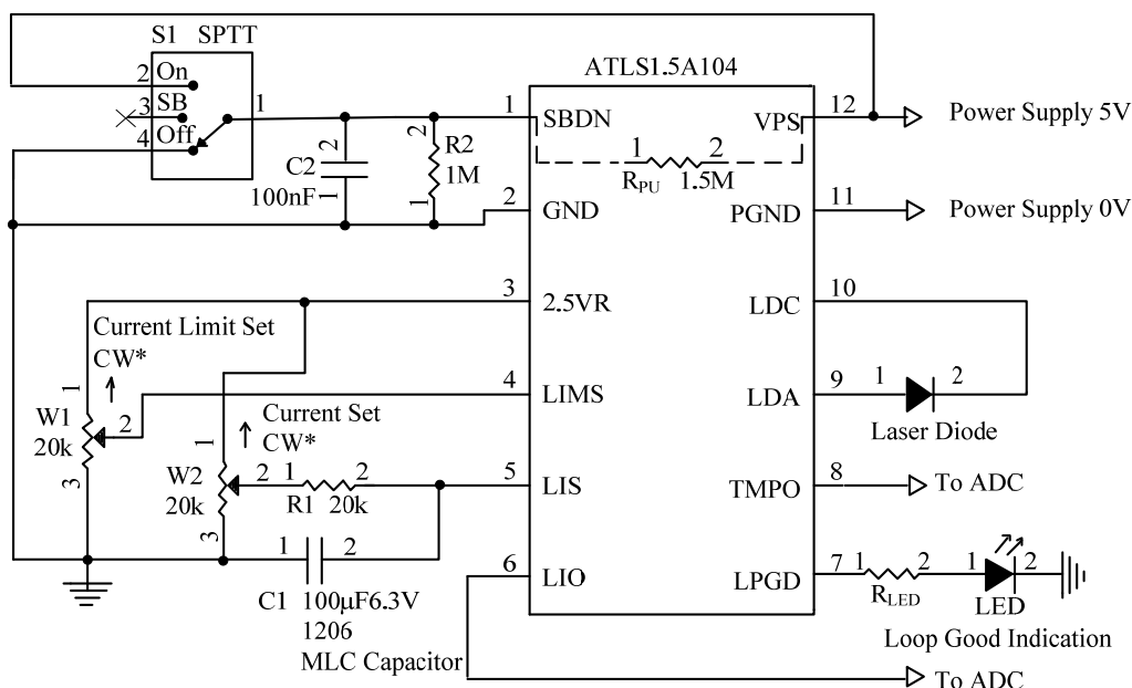
Figure 5.1. Typical Stand-alone CW Operation Schematic for ATLS1.5A104
