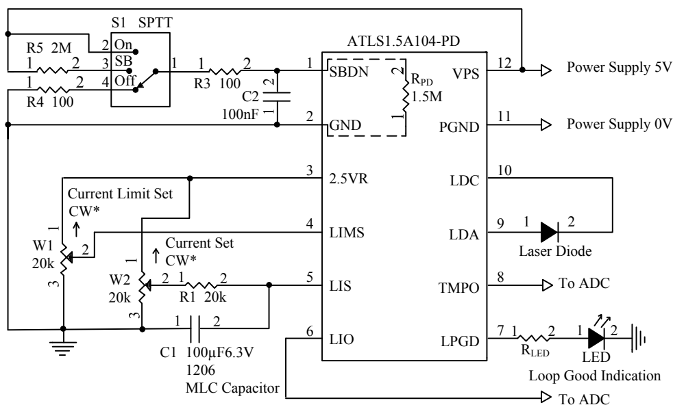
Figure 5.2. Typical Stand-alone CW Operation Schematic for ATLS1.5A104-PD
